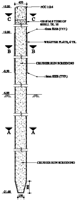
SECTIONAL ELEVATION (SCALE - 1 : 20)
