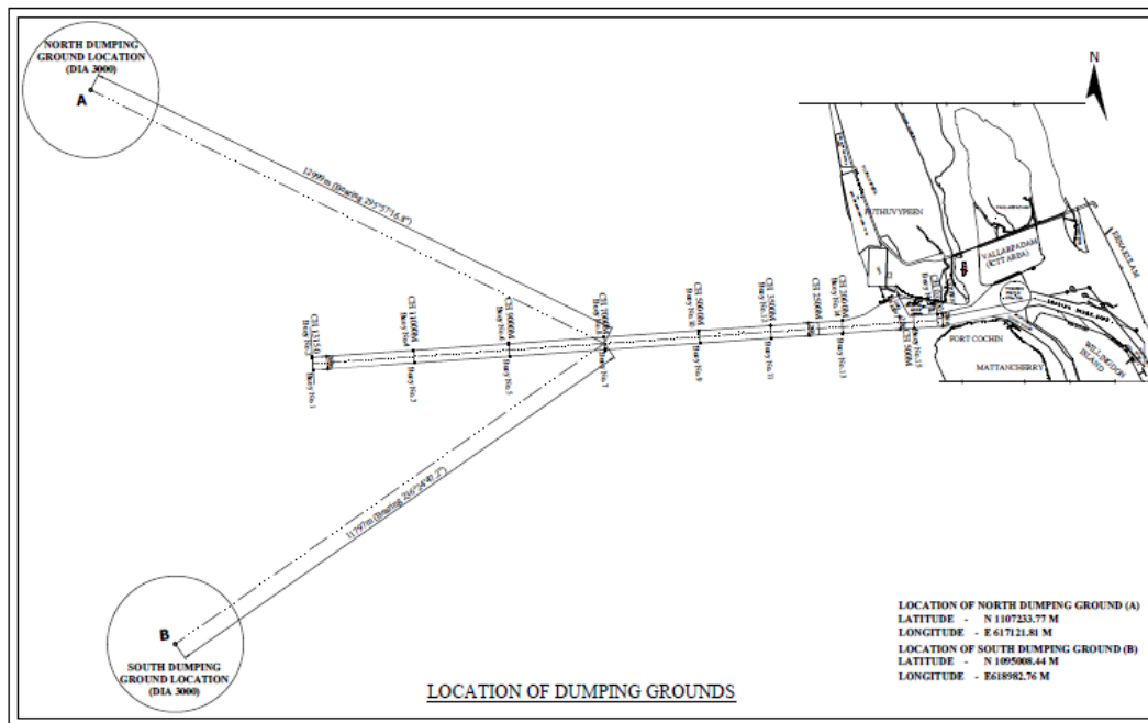
Figure -5: Proposed location for Dredge Spoil Disposal (Dumping Area)
