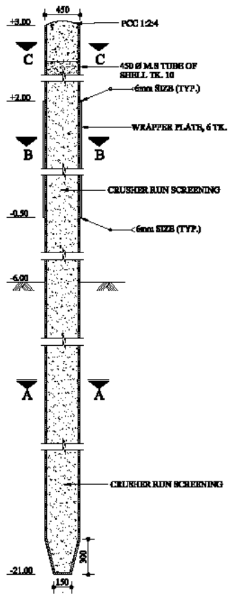
SECTIONAL ELEVATION (SCALE - 1 : 20)
