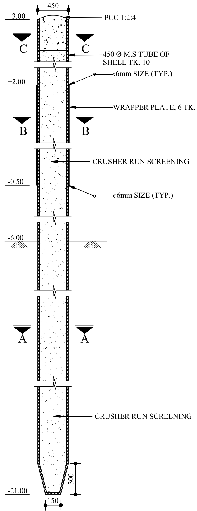
SECTIONAL ELEVATION (SCALE - 1 : 20)
