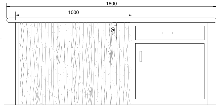
ELEVATION-E2
